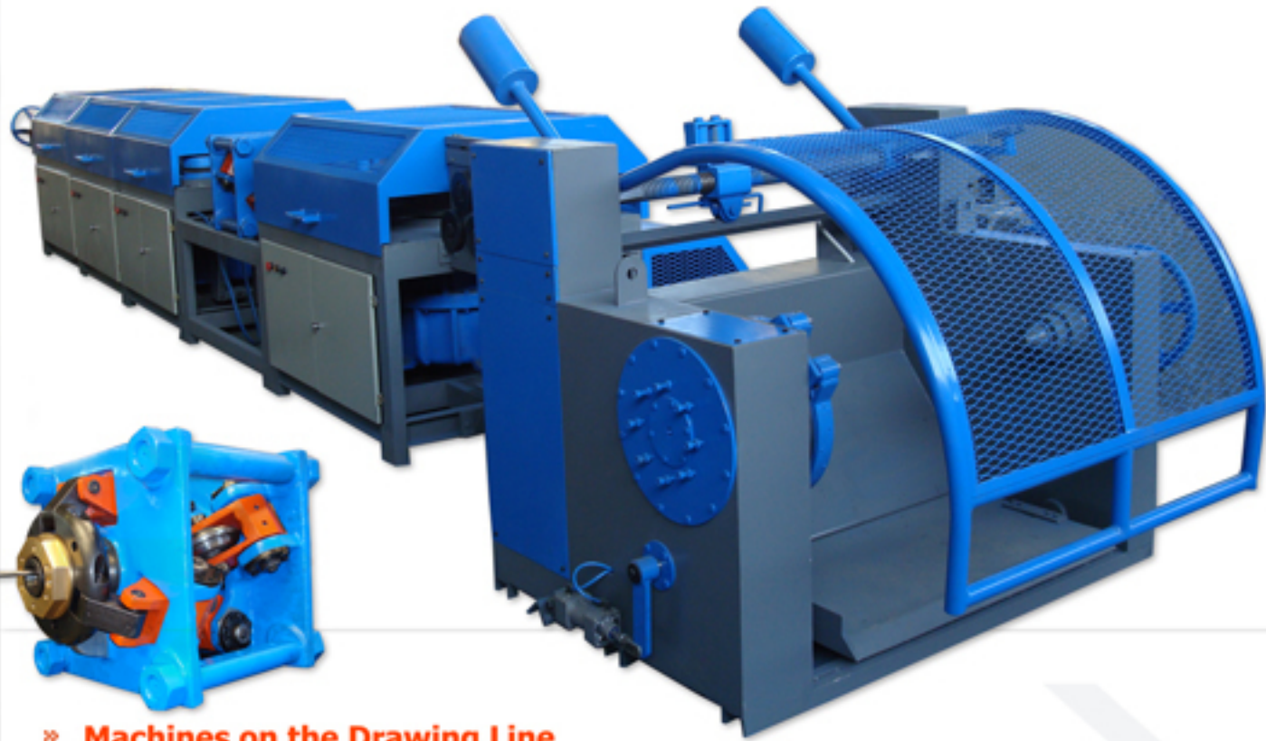
Wire Drawing Line GTCE-9
